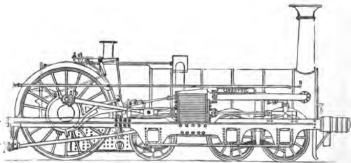
Fig. 59.—"Liverpool," London and North-Western Railway, 1848. (Southern Division, No. 245.)
